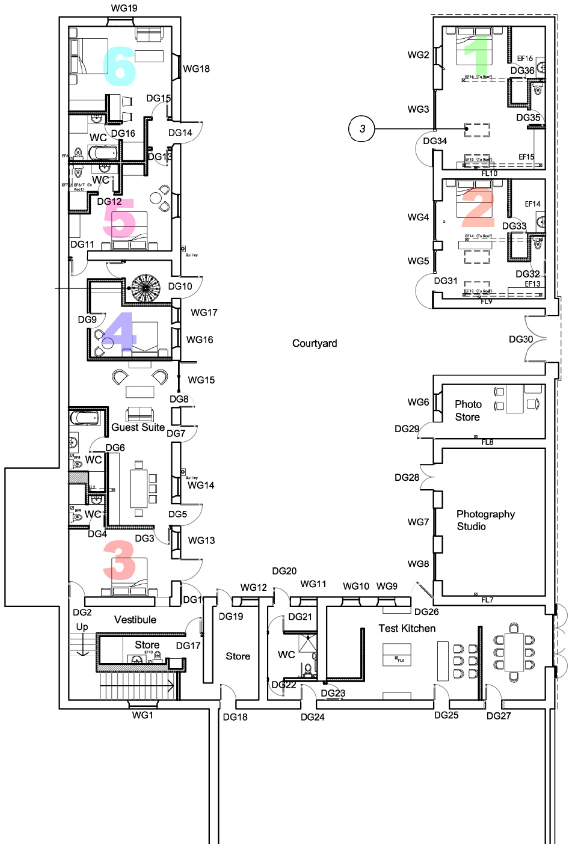
Barn Ground Floor Plan 1:200
